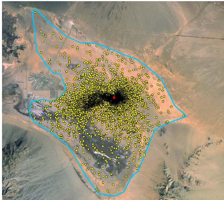
Figure 3. Bristol Dry Lake EC Footprint. The yellow dots represent the 30-min flux values measured by the EC tower (red dot). The light blue line is the EC footprint area.
