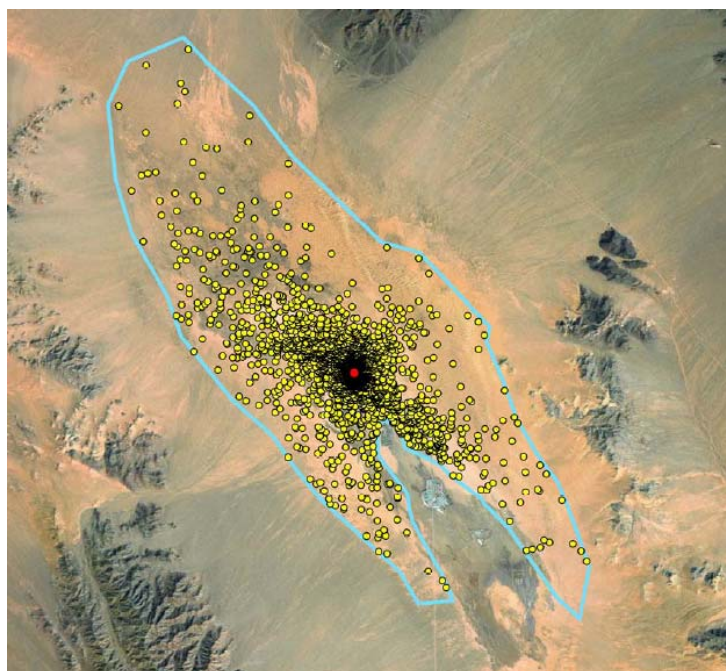
Figure 4. Cadiz Dry Lake EC Footprint. The yellow dots represent the 30-min flux values measured by the EC tower (red dot). The light blue line is the EC footprint area.
